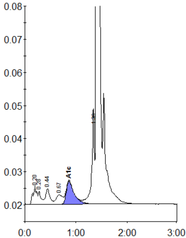
Peak table - ID: 10506381
